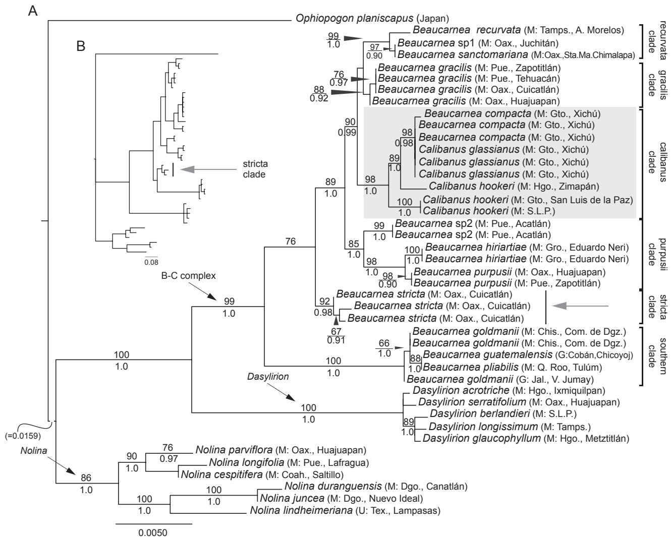
Fig. 3. Maximum likelihood (ML) and Bayesian trees derived from analysis of the concatenated datasets (ITS-trnLF-yefI). A , maximum likelihood phylogram showing high support values for the paraphyly (highlighted by gray rectangle) of Beaucarnea and Calibanus (B-C complex), and the monophyly of Dasyllirion and Nolina . Abbreviations as in Fig. 2. B , Bayesian strict consensus tree. A and B have almost the same topology except for the ambiguous position of B. stricta , highlighted with gray arrows.
